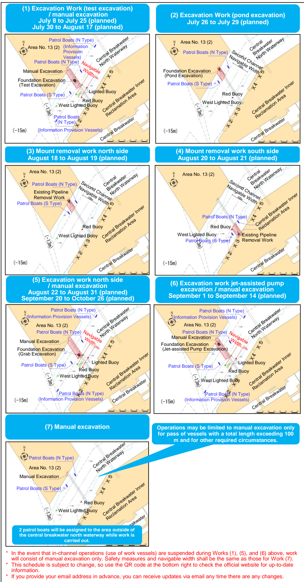
Figure-2 Navigable Lanes for Each Construction Phase
