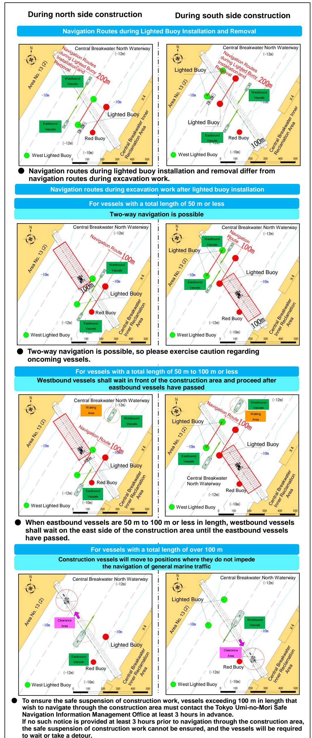
Figure-3 Navigation Methods Near Construction Locations
